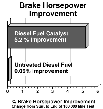
Figure 6: Red Line Diesel Fuel Catalyst improved the average power output of the fleet greater than 5%.
