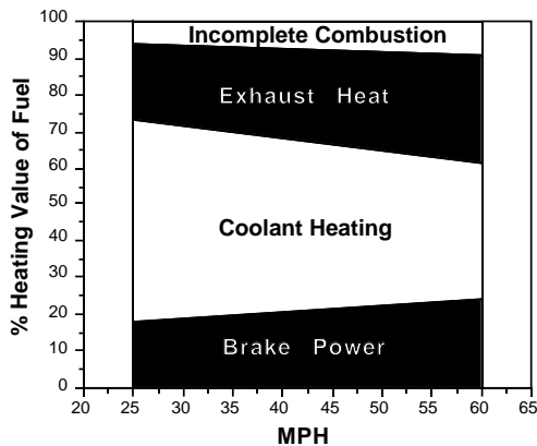
Combustion Heat Distribution
